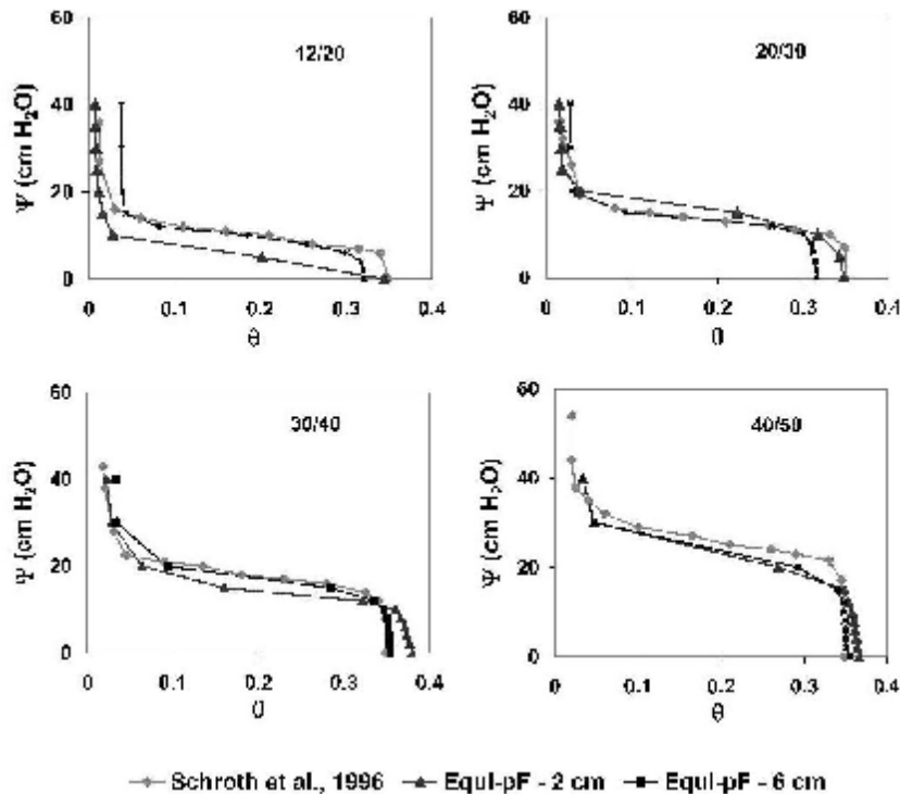
Figure 4. Equi-pf measured drying water retention curves for 2 cm and 6 cm cores, compared with published values from Schroth et al., (1996).
