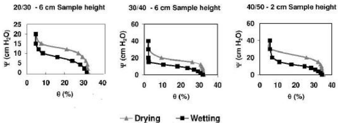
Figure 6. An example set of Equi-pF wetting and drying curves for the homogeneous sand material.
