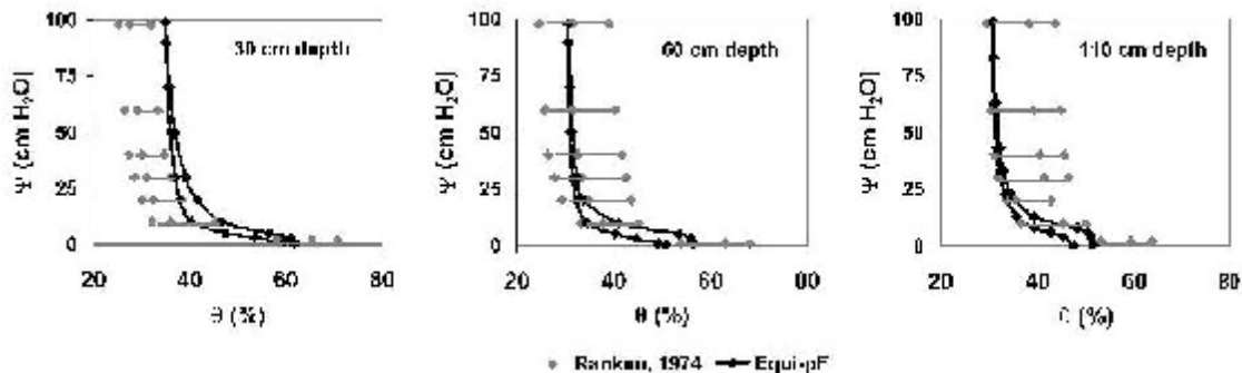
Figure 7. Equi-pF water retention curves for HJA cores compared with range of data developed by Ranken (1974). The bars represent the minimum, mean, and maximum water contents calculated by Ranken (1974) for each of the tension steps, and are representative only of drying conditions.
