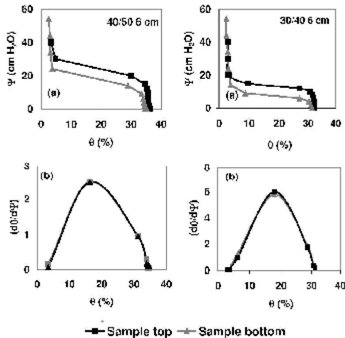
Figure 8. Water retention curves for 6 cm 30/40 and 40/50 grade sand samples with reference points as the top and bottom of the sample. Lower plots are the slope of the water retention curves as change in water content ( d\theta ) per unit change in suction ( d\psi ).
