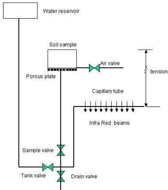
Figure 1. Components of Equi-pF
