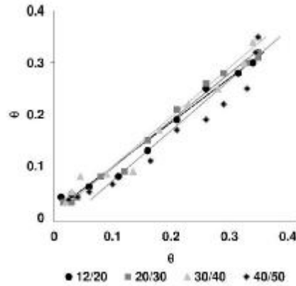
Figure 5. Comparison plots of water content for results from Equi-pF and Schroth et al., (1996). Results from the Equi-pF were interpolated to match the original tension steps utilized by Schroth et al., (1996). Fitted regression lines are included to aid in interpretation.
