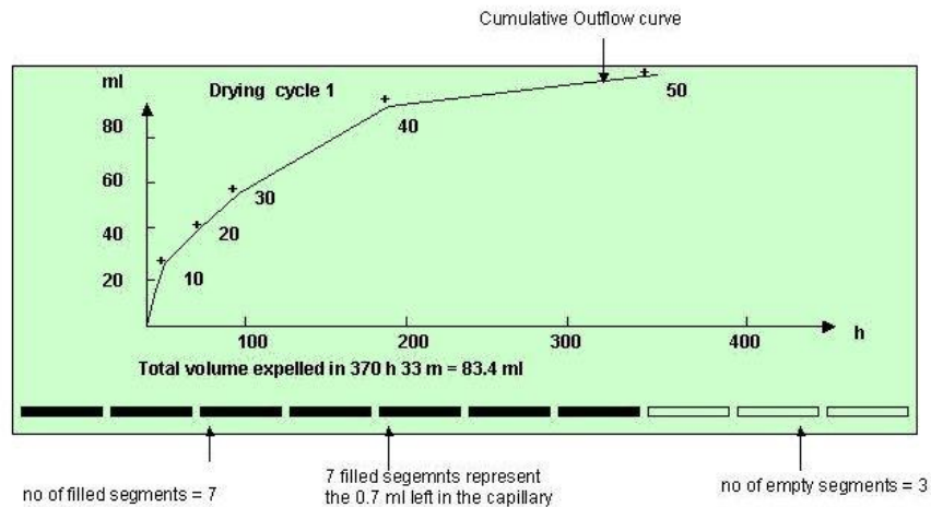
Figure 2. Current progress of a sample run on the Equi-pF is displayed as a cumulative outflow curve. The total volume expelled since the start of the experiment is shown. A similar outflow curve can be displayed for the current tension step as volume out/ln against time.
